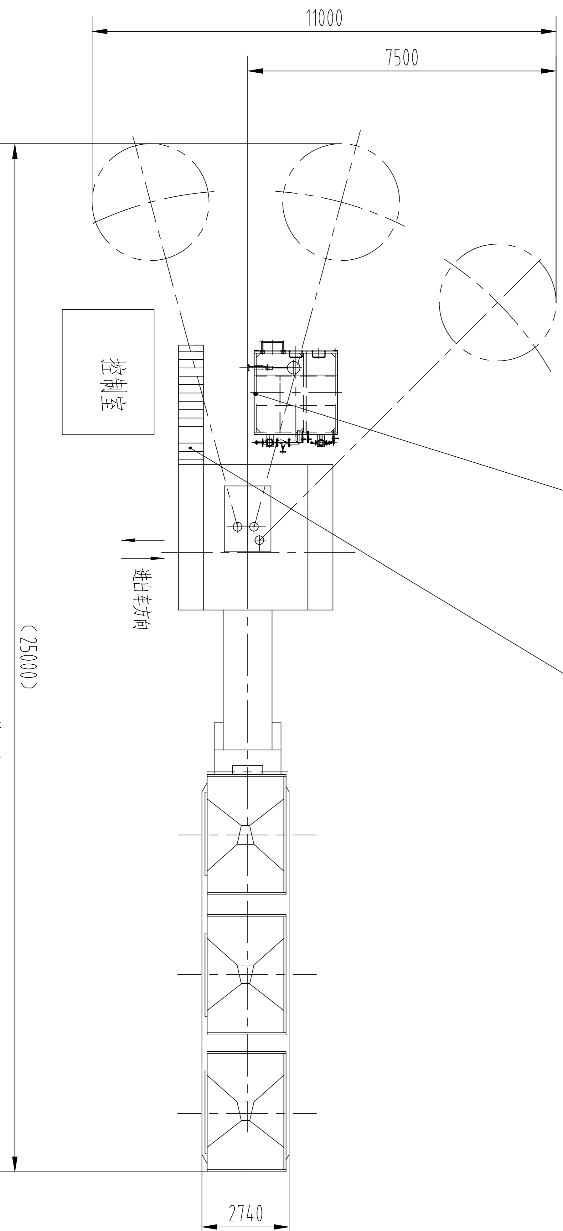
附图：集装HZS25C砼搅拌站简图 Fig.集装HZS25C Concrete batching plant
